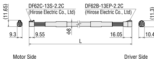
Motor Side
