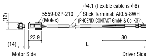
Motor Side
